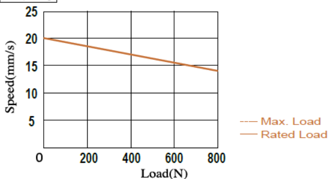
Speed / Load
