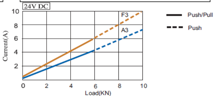
Current/ Load
