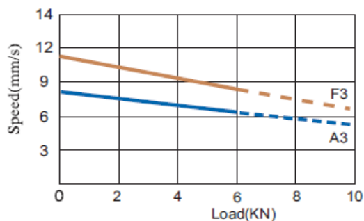
Speed / Load
