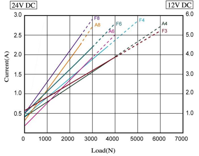
Current / Load
