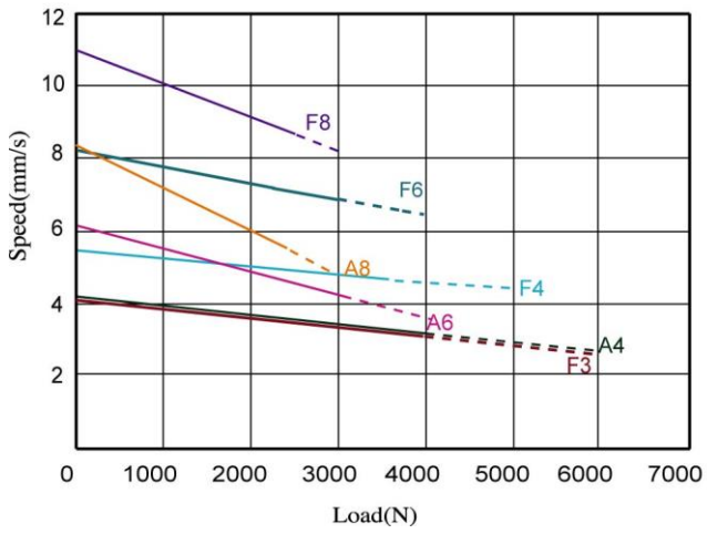
Speed / Load
