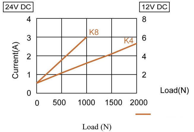
Current / Load
