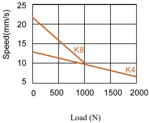
Speed / Load
