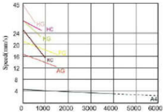
Speed / Load
