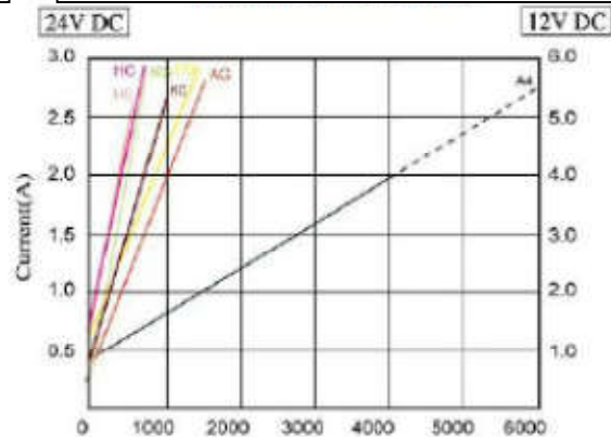
Current / Load
