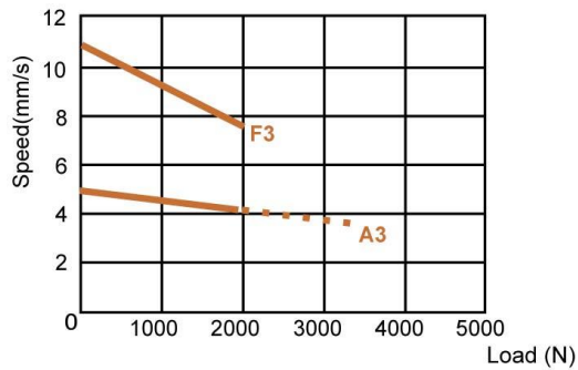
Speed / Load
