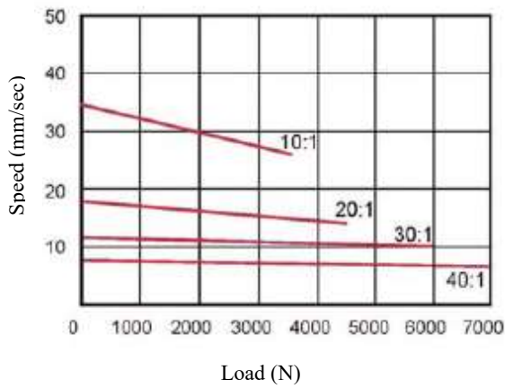
Speed / Load
