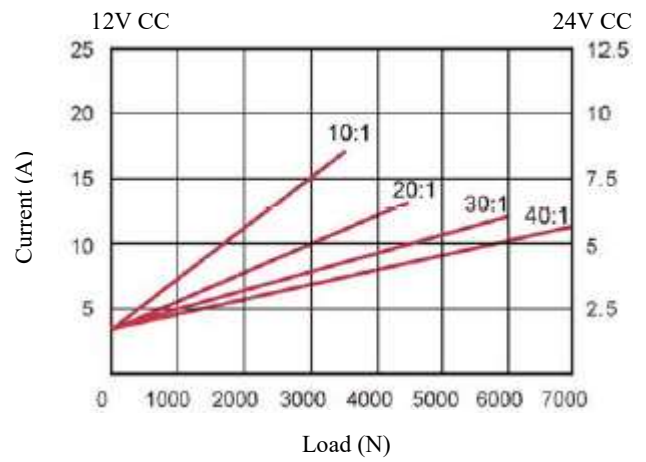
Current / Load
